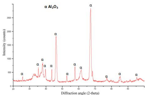
Fig. 2 XRD for \text{Al}_2\text{O}_3 coated “ASTM-SA210-Grade A1” boiler steel
