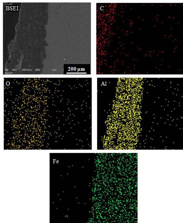
Fig. 4 BSEI and X-ray mapping of the cross-section of \text{Al}_2\text{O}_3 coated “ASTM-SA210-Grade A1” boiler steel
