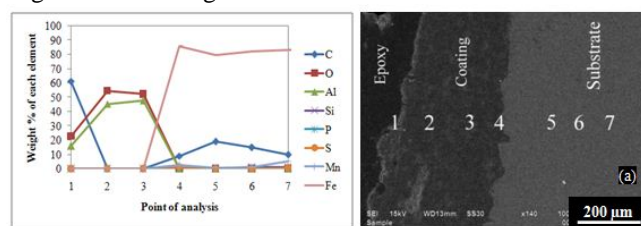
Fig.3 Cross-sectional morphology and variation of elemental composition across the cross- section of \text{Al}_2\text{O}_3 coated “ASTM- SA210-Grade A1” boiler steel
