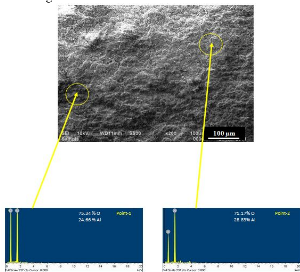
Fig. 1 SEM / EDAX analysis of \text{Al}_2\text{O}_3 coated “ASTM-SA210-Grade A1” boiler steel showing elemental composition (wt.%) at different points, (X200).
