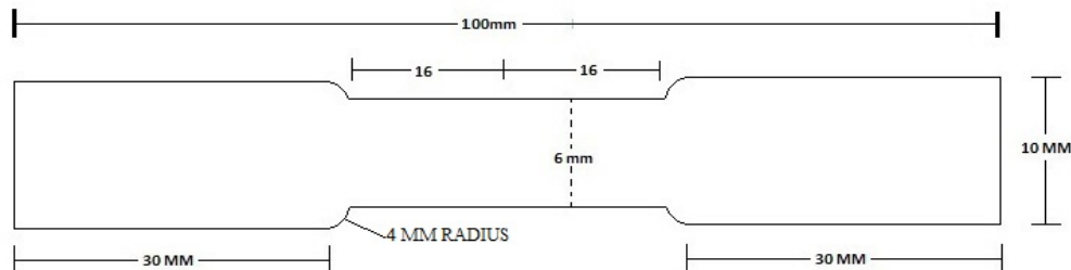
Fig. 1.4: Dimensions of tensile test specimen (in mm)
