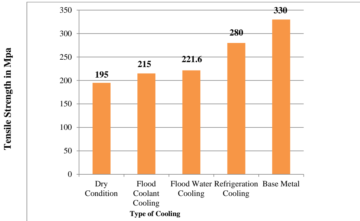
Fig. 1.5: Effect of cooling conditions on the Tensile strength of FSPed samples
