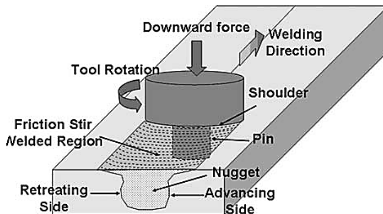
Fig.1.1: Set up of a FSW Process [7].
