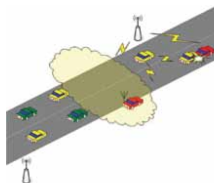
Fig. 2 Spectrum Jamming.
