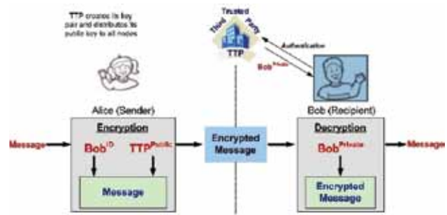
Fig. 6 Identity-Based Encryption.
