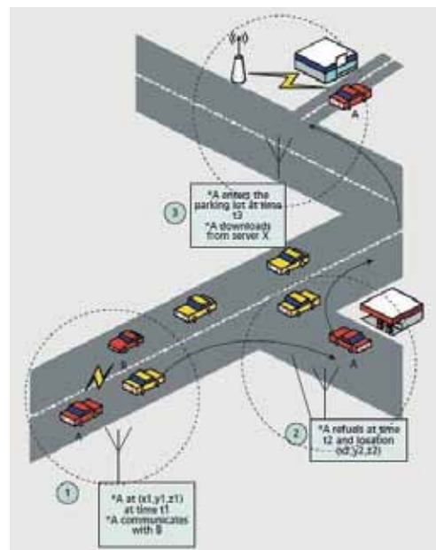
Fig. 4 Privacy Violation
