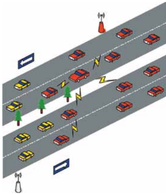
Fig. 3 Message Forgery.
