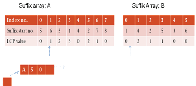
Fig. 7 Insertion of DE(A,5,0)
