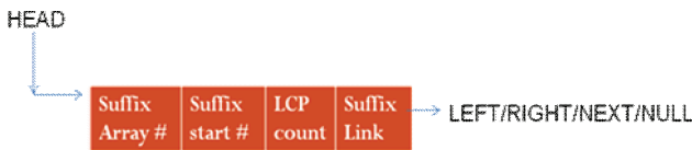
Fig. 4 Node of Compressed suffix tree
