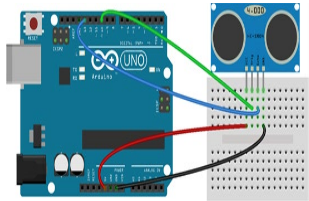
Fig. 1 Full Circuit Connection
