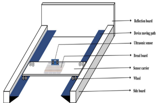
Fig. 2 Main Frame of the Machine
