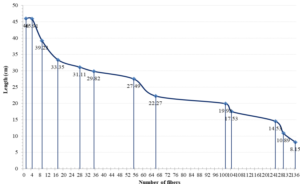
Fig. 6 Graph of Number of Fibers vs. Fiber Length for Sample
