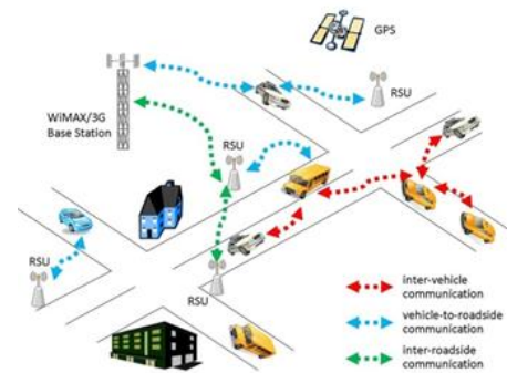
Fig. 1 An Illustration of the VANETs [2]
